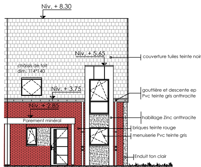
Façade Principale
